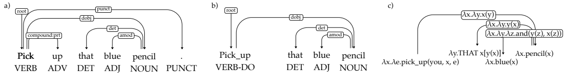
Figure 2: (a) UD parse; (b) tree transformation to subcategorize verb POS, remove punctuation, and combine verb with its particle; (c) LF assignment to nodes and edges.
