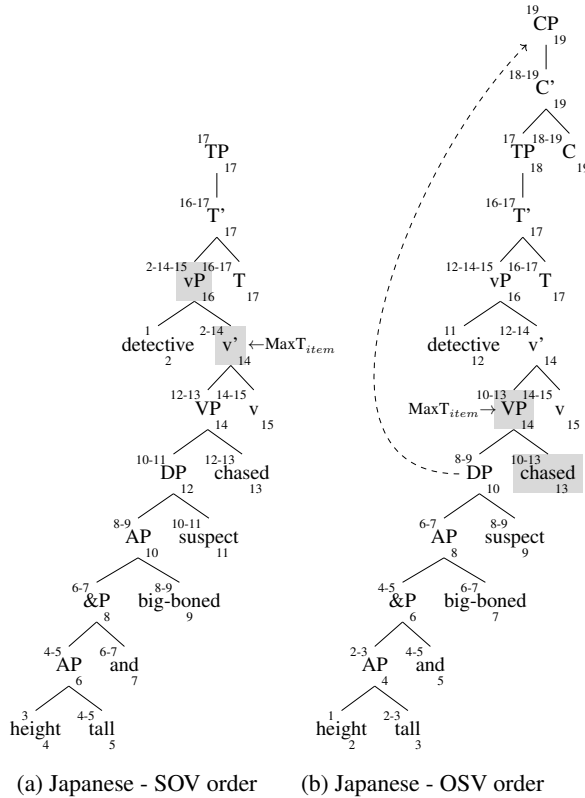
Figure 2: Tree annotations for long-before-short preference
