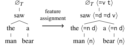
Figure 3: Feature assignment transduction
