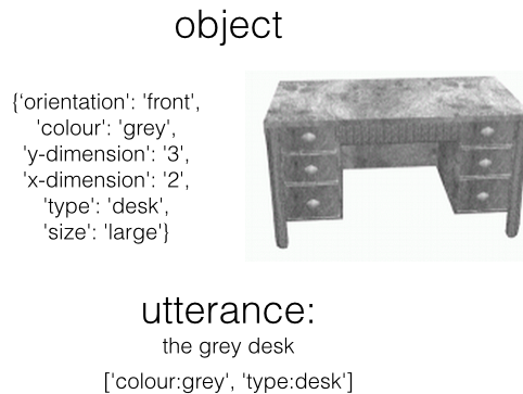
Figure 4: An example target entity from the furniture domain, along with its coding as a dictionary, and the human generated referring expression for it in a context of other images.
