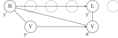
Figure 6: Output of the transduction in Table 1 given Fig. 5 as input; i' indicates a surviving copy of node i from Fig. 5.
