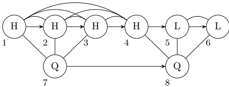
Figure 5: An example QR of the sequence \hat{V}\hat{V} .
