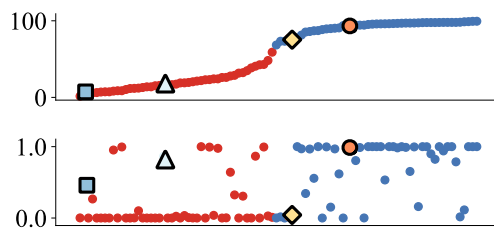
Figure 4: Top : mean truth score given by humans on 96 statements. False statements colored red, true blue; statements from Table 1 overlaid. Bottom : P(\text{true}) assigned by the best probing classifier (XLNet + [CLS]).
